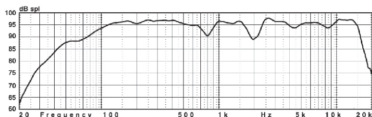
on axis response (2.83v@1m, free-field conditions)
